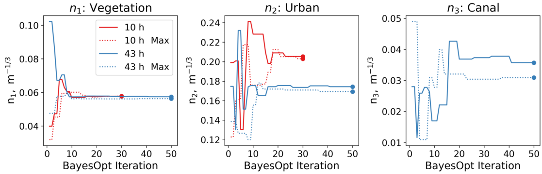
Figure S123. Bayesian optimization convergence plots for each Manning's n in the 10-h, 10-h Max, 43-h, and 43-h Max experiments.
